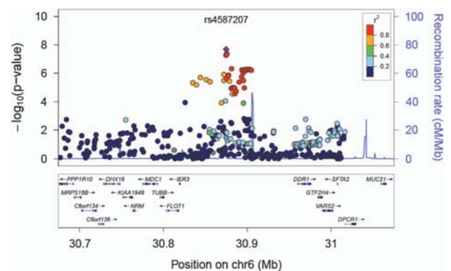
Figure 3. Chromosome 6 regional association plot for usual sleep duration in cohorts of European descent. Figure was constructed using the Broad Institute SNAP tool ( http://www.broadinstitute.org/mpg/snap/ ).
