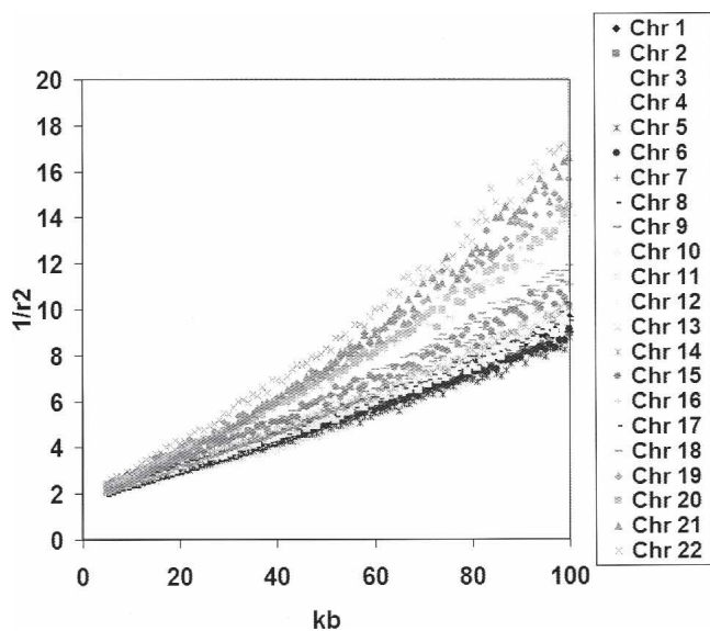
Figure 1. Reciprocal of r^2 plotted against physical distance for each of the 22 autosomes for the CEU population. The X-axis shows the physical distance in kilobases and the Y-axis shows 1/\text{mean}(r^2) . The mean value of r^2 was calculated in 1 kb bins.
